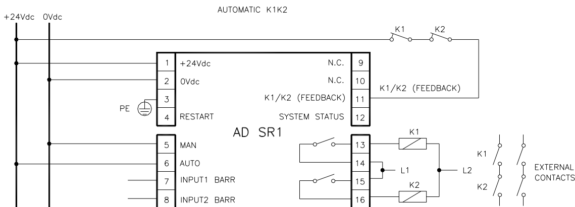
Figure 3 Automatic functioning with K1K2 relays
