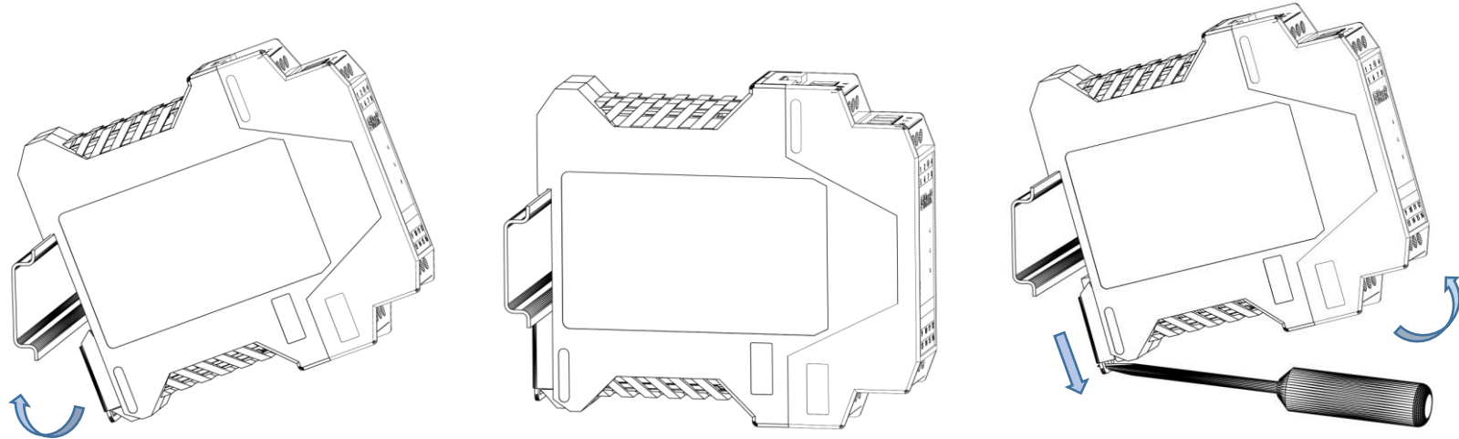
Figure 1 – Montaggio-smontaggio meccanico / Mechanical assembly-disassembly
